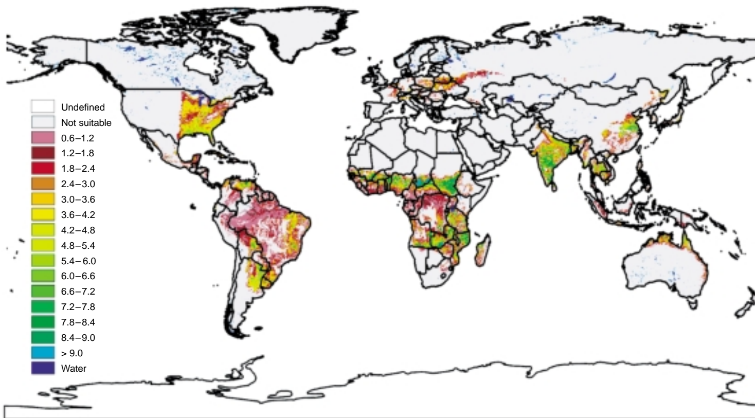
Plate D. Expected grid-cell output a per hectare for 120 day rain-fed grain maize (high level of inputs). a Grid-cell output differs from yields; it accounts for per hectare production of total land of individual grid-cells, including not suitable areas.
