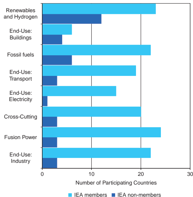
Figure 24.13 | Examples of international technology cooperation via IEA agreements, by participating countries (IEA members and non-members), number of agreements covered (left panel) and number of participating countries (right panel). Note in particular the relative sparse participation from developing countries, which is less surprising considering the exclusive OECD membership of IEA. Source: based on IEA, 2010.
