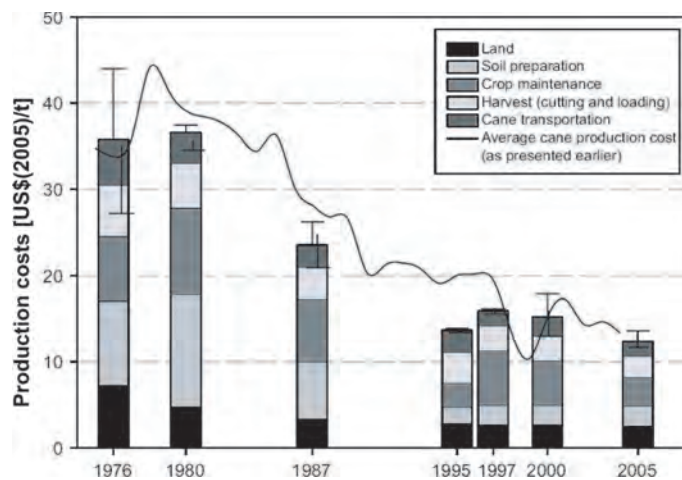
Figure 24.8 | Decomposition of cost components and their improvements for Brazilian ethanol (cane production only). Source: van den Wall Bake et al., 2009.
