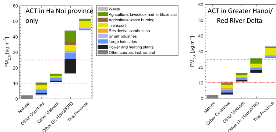
Figure 12: Source contribution to population-weighted PM 2.5 in the Ha Noi province in 2030 for the 'Advanced Technology' set of measures applied to Ha Noi province (left panel) and in all of Northern Vietnam (right panel)
