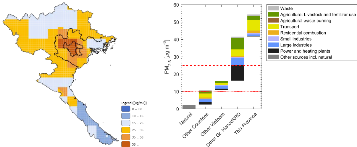
Figure 13: Ambient concentrations of PM 2.5 resulting from the substitution of five percent of coal by rice straw residues in the power sector (co-firing) in 2030 and the source contribution in the Ha Noi province
