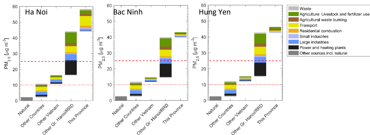
Figure 10: Source apportionment for the current legislation baseline projection in 2030. The graph shows the contributions to population-weighted PM2.5 concentrations in the Ha Noi province (left panel), Bac Ninh province (centre panel) and Hung Yen province (right panel)
