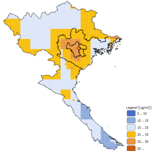
Figure 5: Ambient levels of PM2.5 modelled for 2015 (annual mean concentrations, \mu\text{g}/\text{m}^3 )
