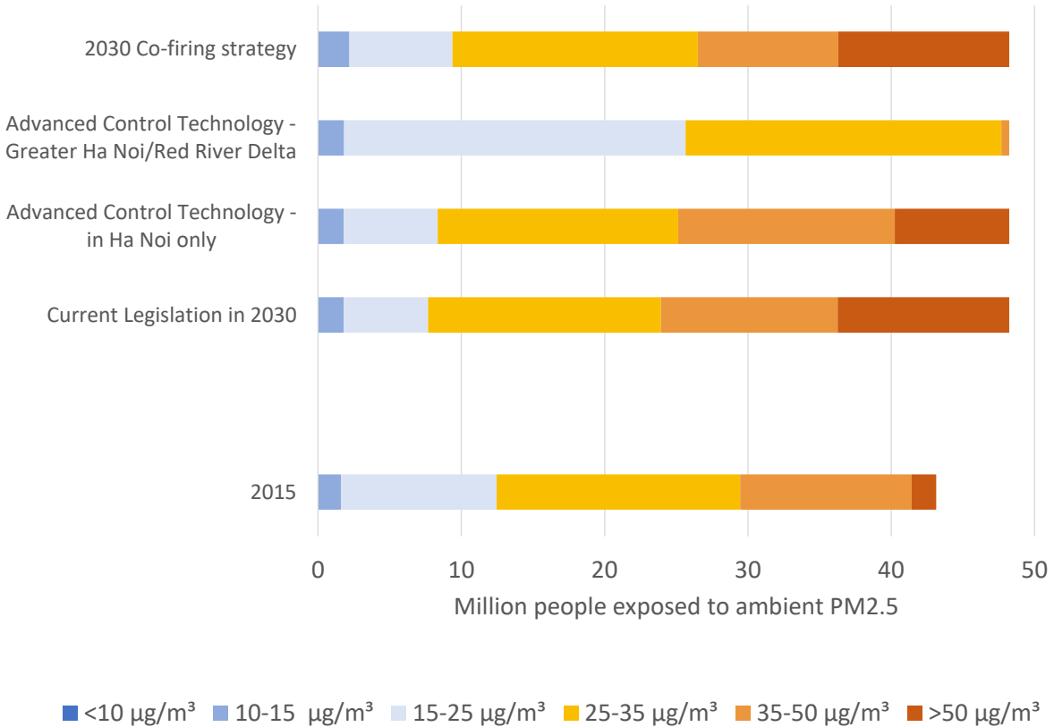
Figure 15: Distribution of population exposure to ambient PM2.5 in northern Vietnam for the different emission scenarios
