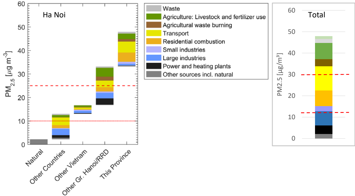
Figure 7: Sources of PM 2.5 concentrations (population-weighted annual mean) in the Ha Noi province in 2015. The x-axis distinguishes the spatial origin of PM 2.5 , i.e., (from right to left:) (i) emission sources within the same province, (ii) sources in the other provinces in the Greater Ha Noi/Red River Delta region, (iii) Vietnamese provinces outside the Greater Ha Noi/Red River Delta region, (iv) sources in other countries and international shipping, and (v) natural sources (sea salt, soil dust). The y-axis indicates the amounts originating from emissions of the different economic sectors. The red lines indicate Vietnam’s national air quality standard (25 \mu\text{g/m}^3 ) and the global WHO air quality guideline for PM 2.5 (10 \mu\text{g/m}^3 ).
